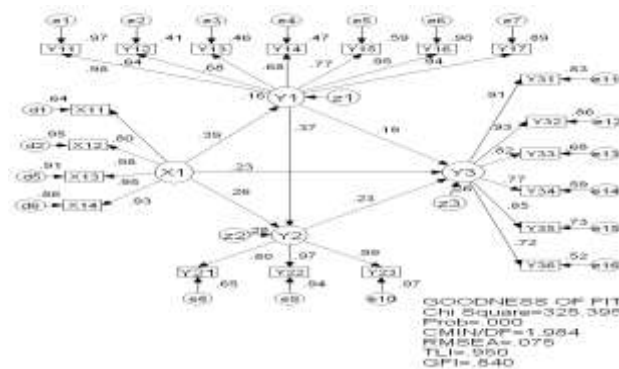
FIGURE 2 FULL MODEL SEM ANALYSIS
