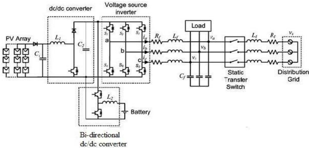
FIGURE 8 THE PV SYSTEM TO GRID NETWORK
