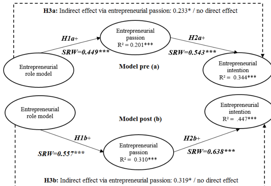
Figure-2 SEM MODEL RESULTS: STANDARDIZED REGRESSION WEIGHTS FOR THE HYPOTHESES (N = 426)
