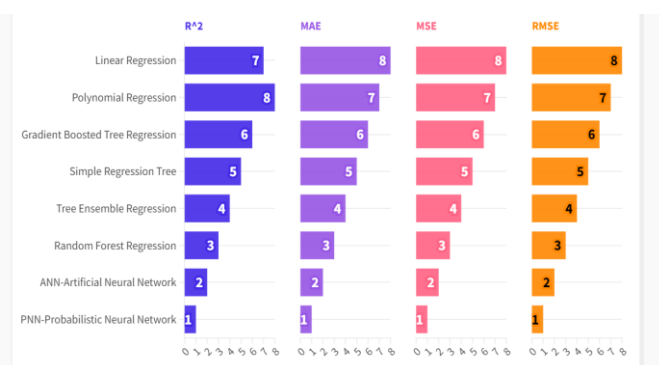
Figure 9 STATISTICAL ERRORS OF THE MACHINE LEARNING ALGORITHMS
