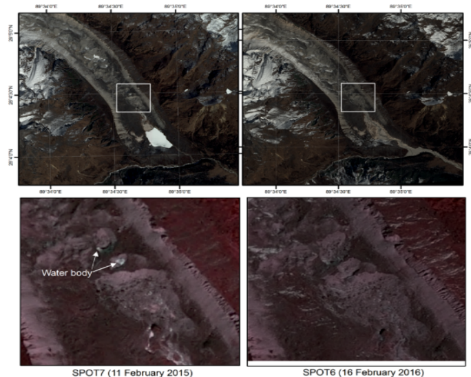
Figure 3. Pre (left) and post (right) GLOF event SPOT images of Lemthang Tsho. Bottom images clearly show the emptying of two supraglacial ponds, which ultimately resulted in the outburst.
