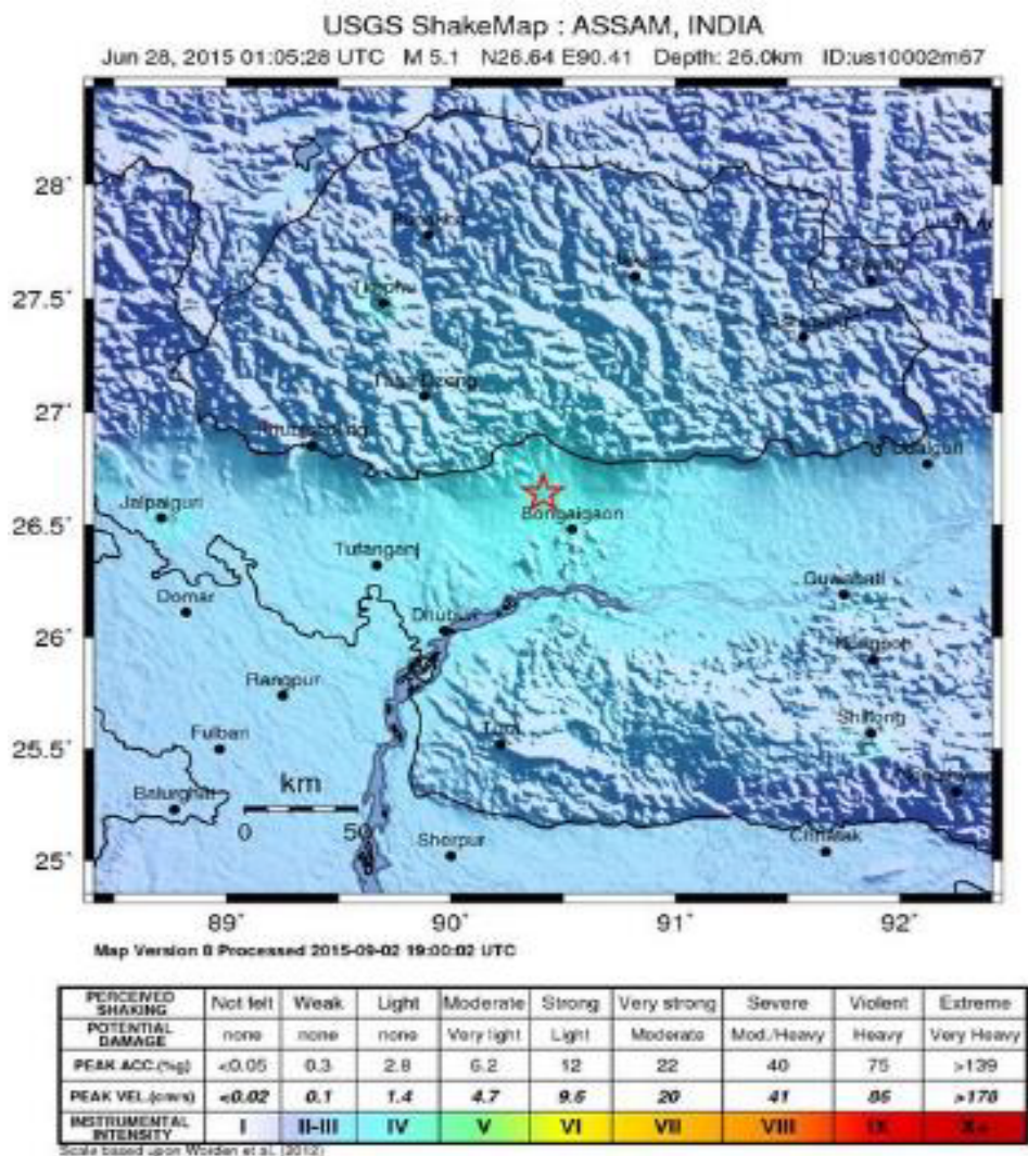
Figure 4. Shake intensity map of M5.1 earthquake that struck Assam on the morning of 28 June 2015 (Source: USGS).
